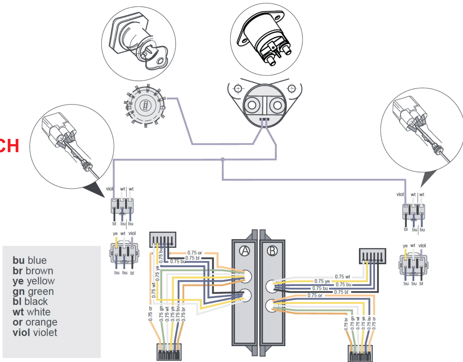
Figure 3.4: Easy start function electronic module
